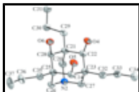
Fig. 2. Molecule B of the title compound with displacement ellipsoids drawn at the 50% probability level. Hydrogen atoms have been omitted for clarity.
