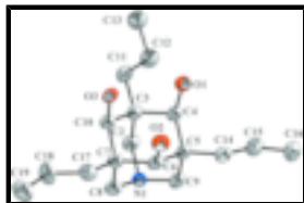
Fig. 1. Molecule A of the title compound with displacement ellipsoids drawn at the 50% probability level. Hydrogen atoms have been omitted for clarity.
